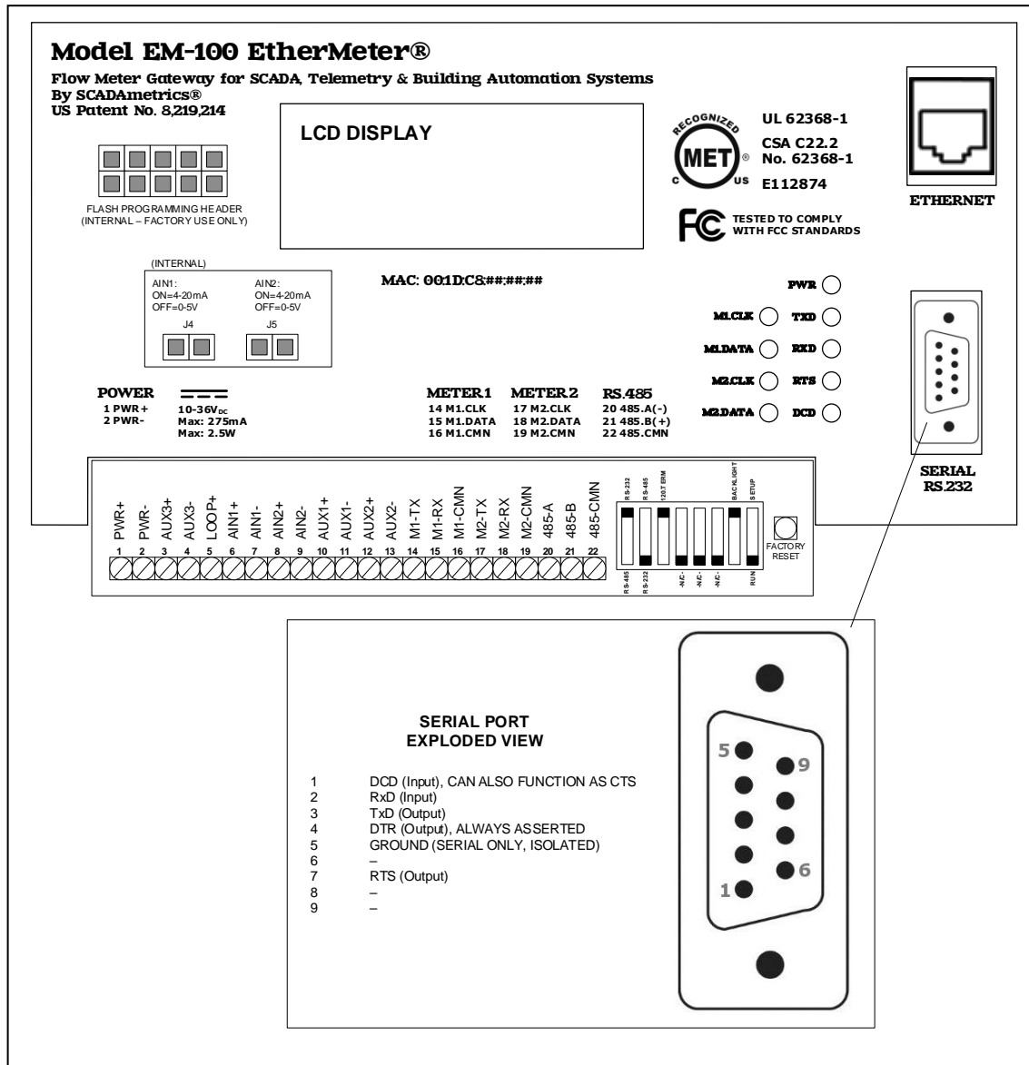
Figure 4A. Electrical Interface
