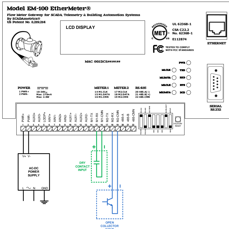
Figure 9A. Example Pulse Signal Hookups to EtherMeter
