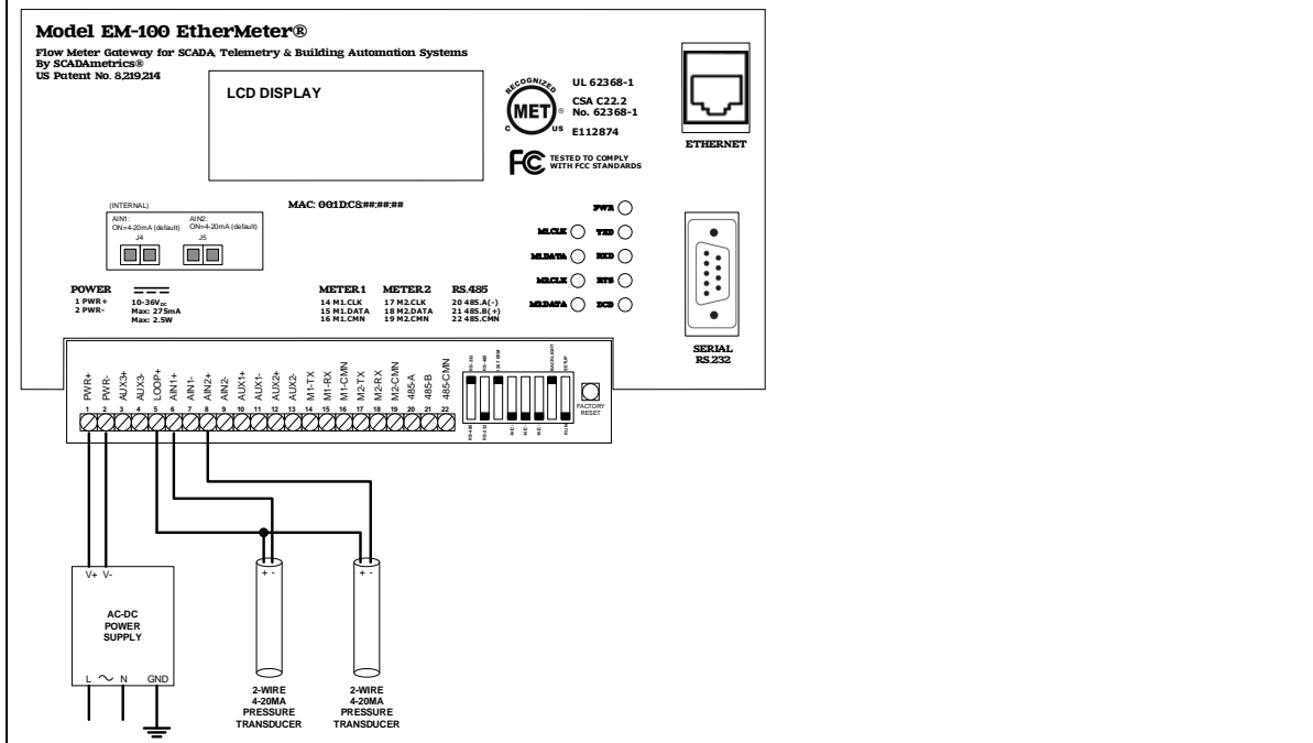
Figure 12A. Correct 4-20mA Analog Input Wiring.
