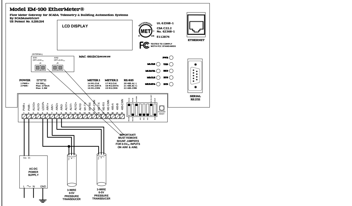
Figure 12B. Correct 0-5V Analog Input Wiring.
