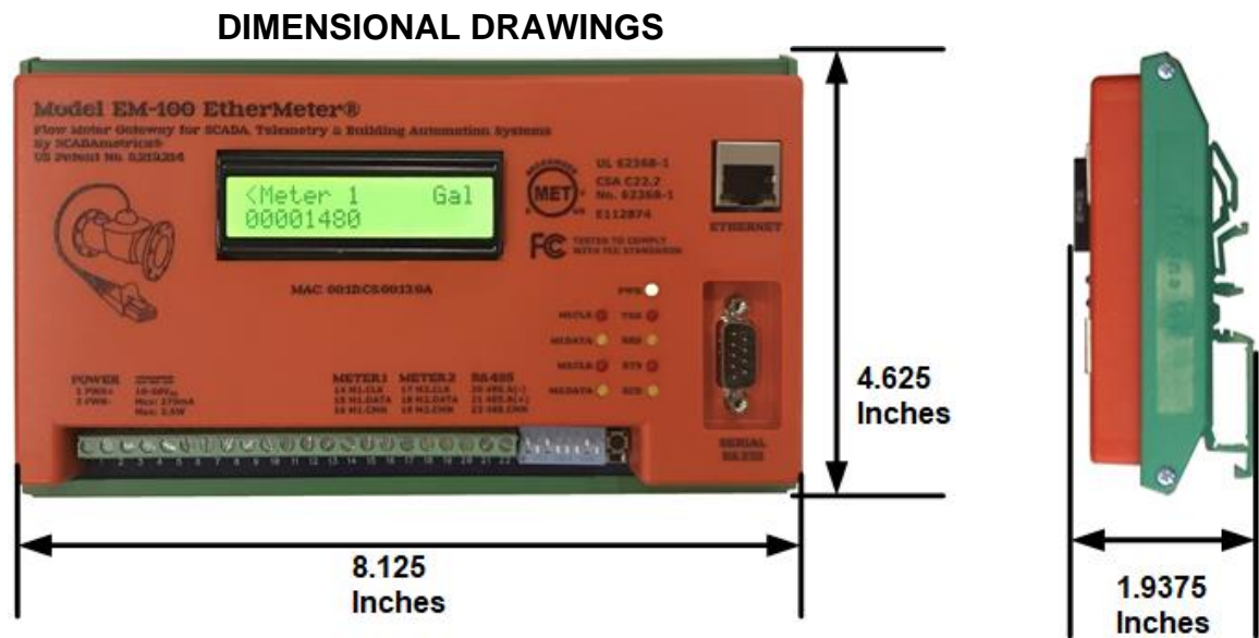
Figure 3A. Dimensional Drawing
