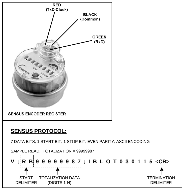
Sensus ICE™ – Register Diagram.
